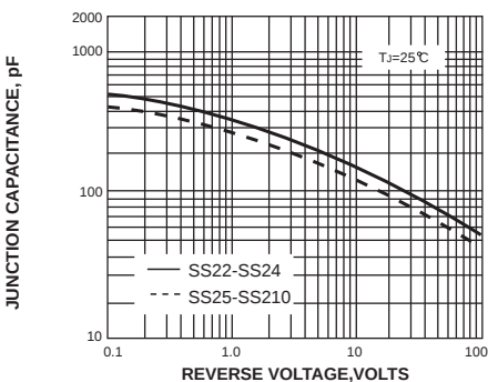
FIG. 5-TYPICAL JUNCTION CAPACITANCE
