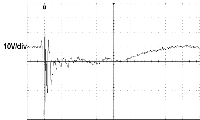
ESD clamping
