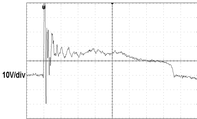
ESD clamping
